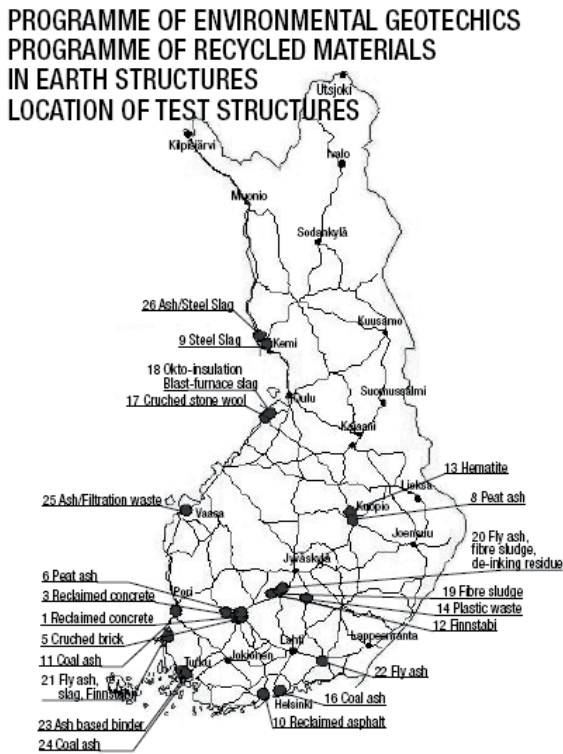
Figure 1.1. By-products and recycled materials in earth works -project of Tekes in connection with location of executed projects.
